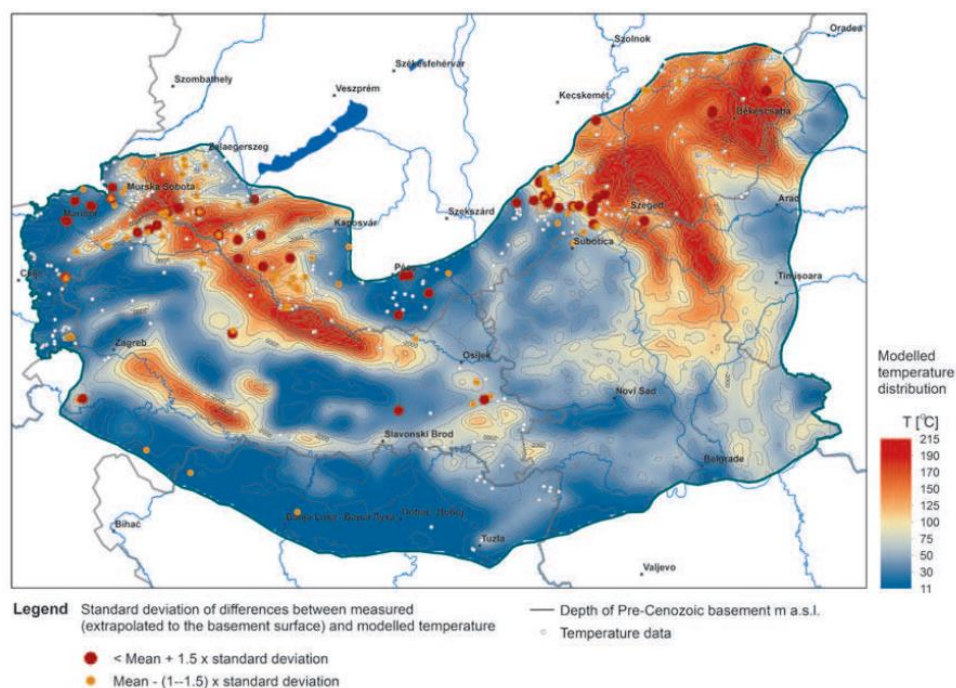
Figure 19: Geothermal potential map of the basement reservoirs, comparison of the temperature values estimated.
