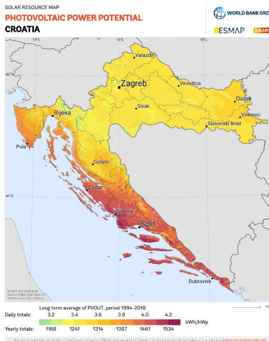
Figure 17: Photovoltaic energy potential 2019. Source: solargis.com
